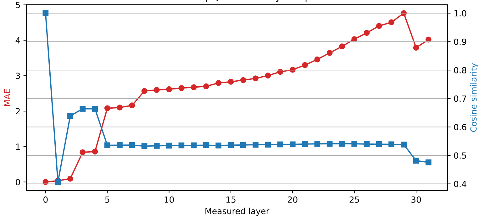
Phi-3-mini-4k-instruct | Quantized layer 0 | float32 \rightarrow int2
