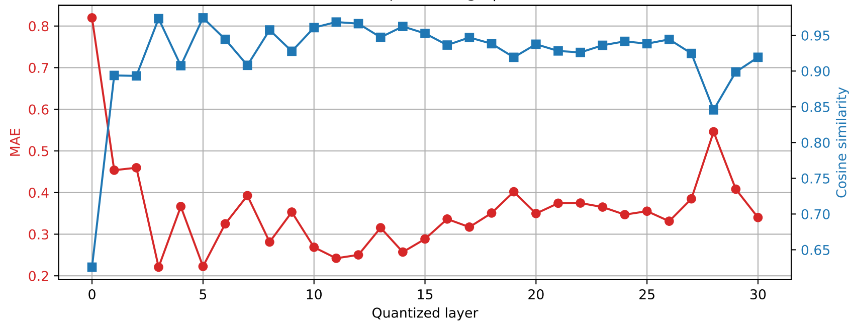
Phi-3-mini-4k-instruct | Prompt 1 Final RMSNorm output damage | float32 → int2
