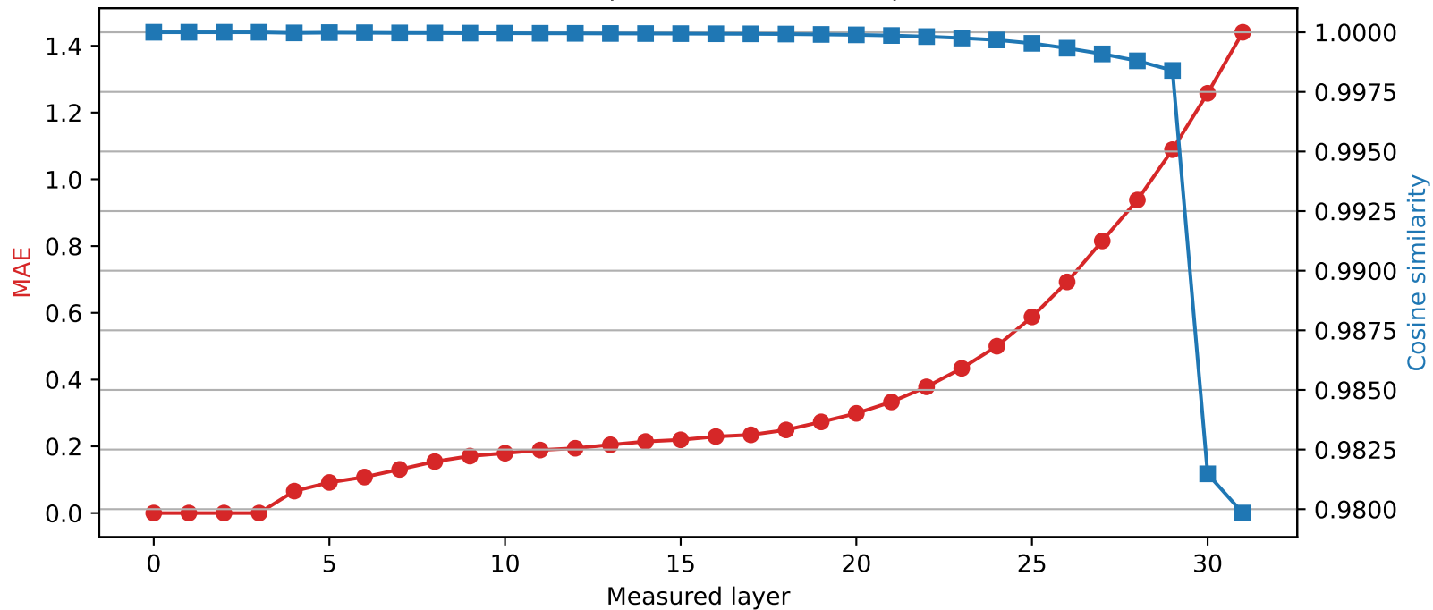
Phi-3-mini-4k-instruct | Quantized layer 3 | float32 \rightarrow int2
