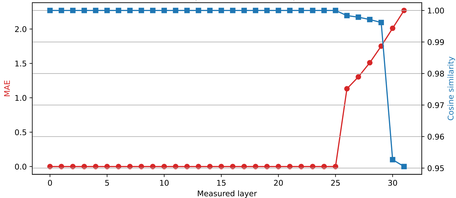
Phi-3-mini-4k-instruct | Quantized layer 25 | float32 \rightarrow int2
