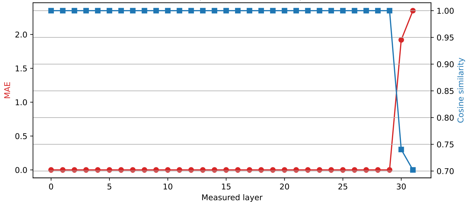
Phi-3-mini-4k-instruct | Quantized layer 29 | float32 \rightarrow int2
