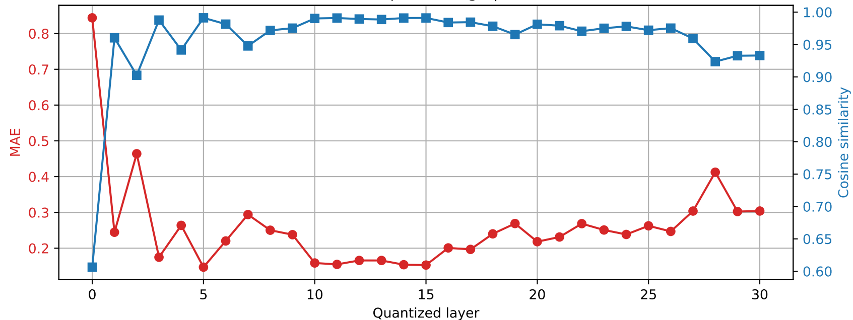
Phi-3-mini-4k-instruct | Prompt 2 Final RMSNorm output damage | float32 \rightarrow int2
