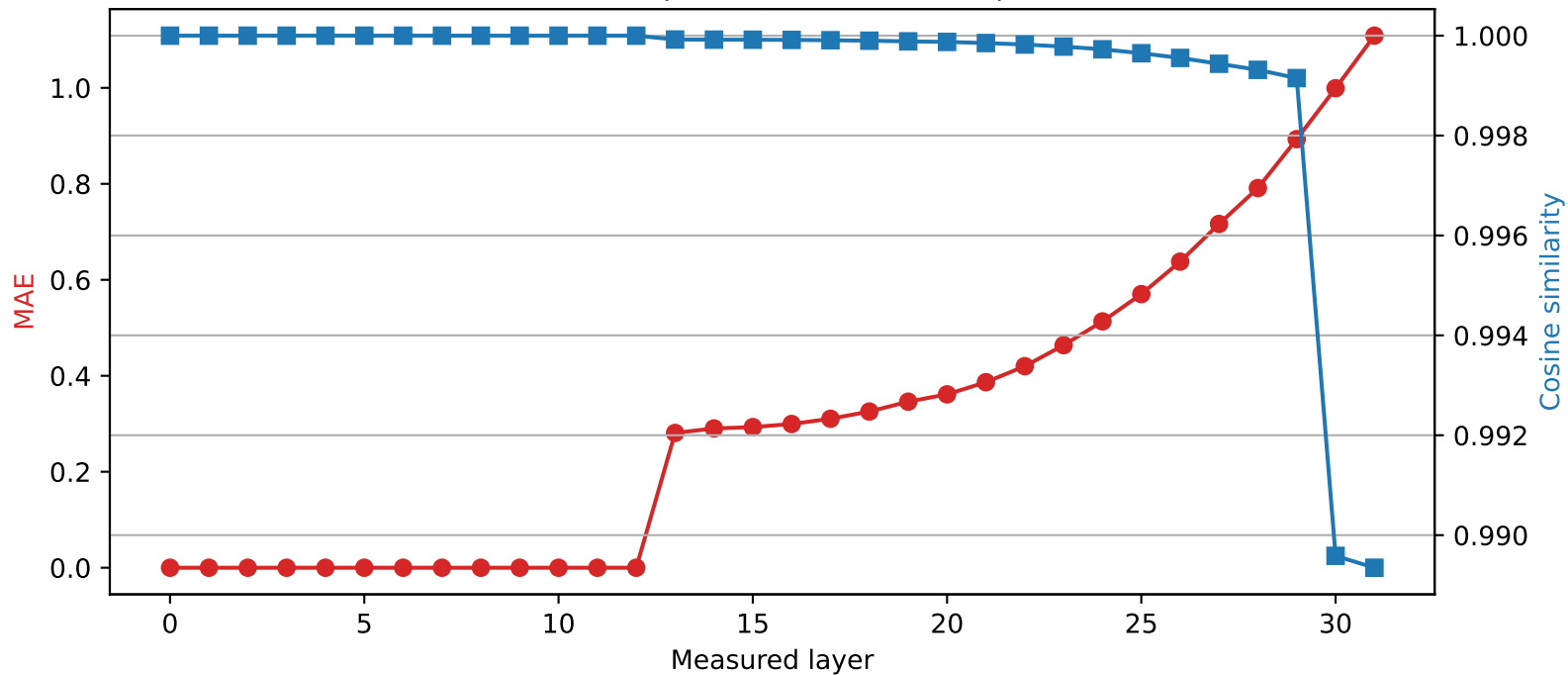
Phi-3-mini-4k-instruct | Quantized layer 12 | float32 \rightarrow int2
