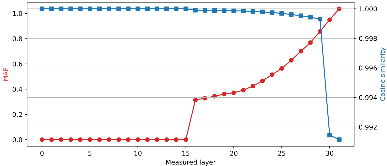
Phi-3-mini-4k-instruct | Quantized layer 15 | float32 \rightarrow int2
