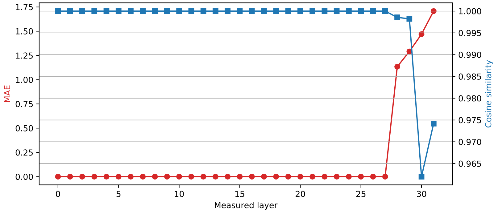
Phi-3-mini-4k-instruct | Quantized layer 27 | float32 \rightarrow int2
