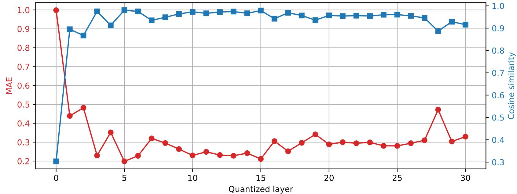
Phi-3-mini-4k-instruct | Prompt 3 Final RMSNorm output damage | float32 \rightarrow int2
