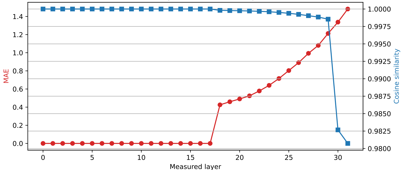
Phi-3-mini-4k-instruct | Quantized layer 17 | float32 → int2
