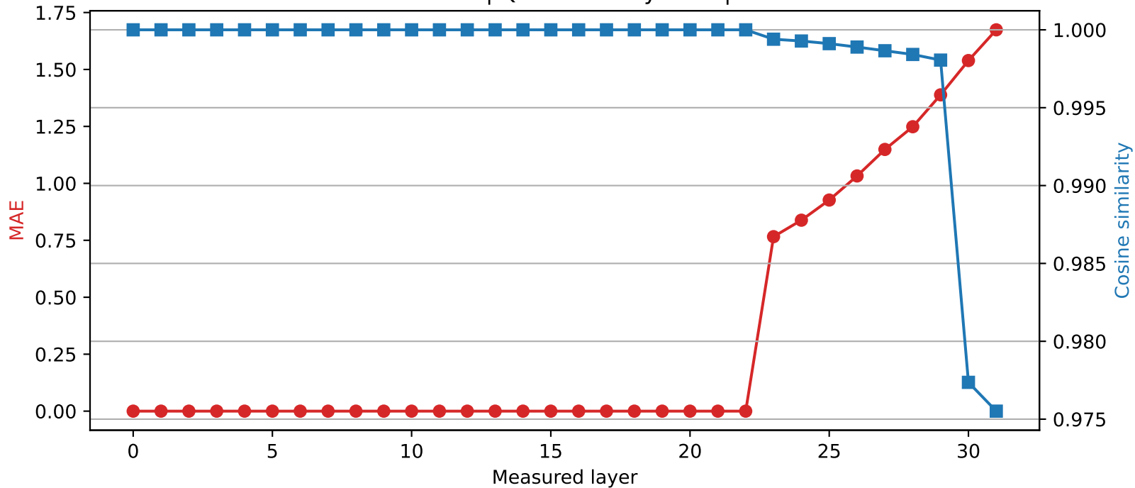
Phi-3-mini-4k-instruct | Quantized layer 22 | float32 \rightarrow int2
