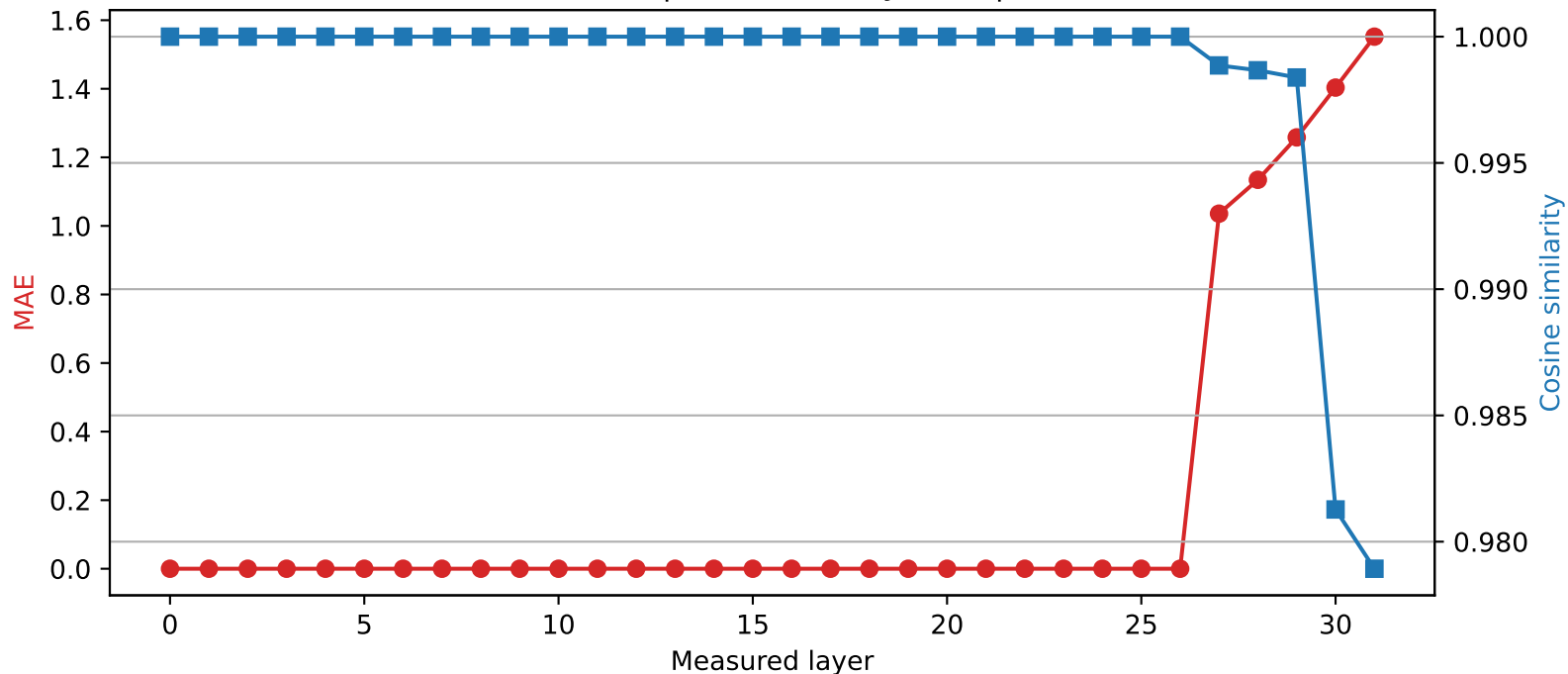
Phi-3-mini-4k-instruct | Quantized layer 26 | float32 \rightarrow int2
