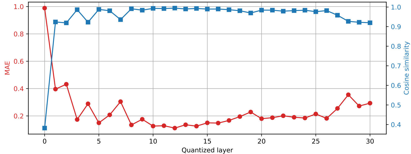
Phi-3-mini-4k-instruct | Prompt 4 Final RMSNorm output damage | float32 \rightarrow int2
