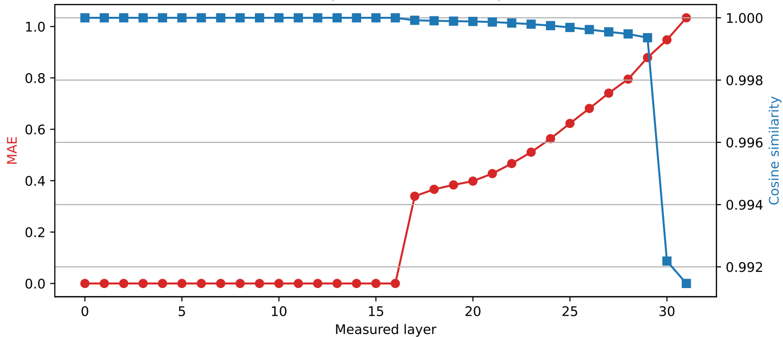
Phi-3-mini-4k-instruct | Quantized layer 16 | float32 \rightarrow int2
