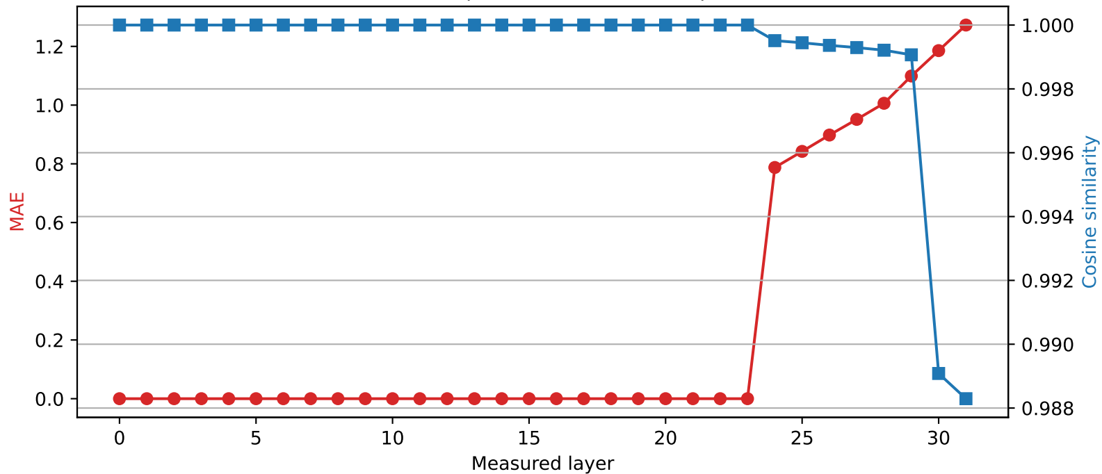
Phi-3-mini-4k-instruct | Quantized layer 23 | float32 → int2
