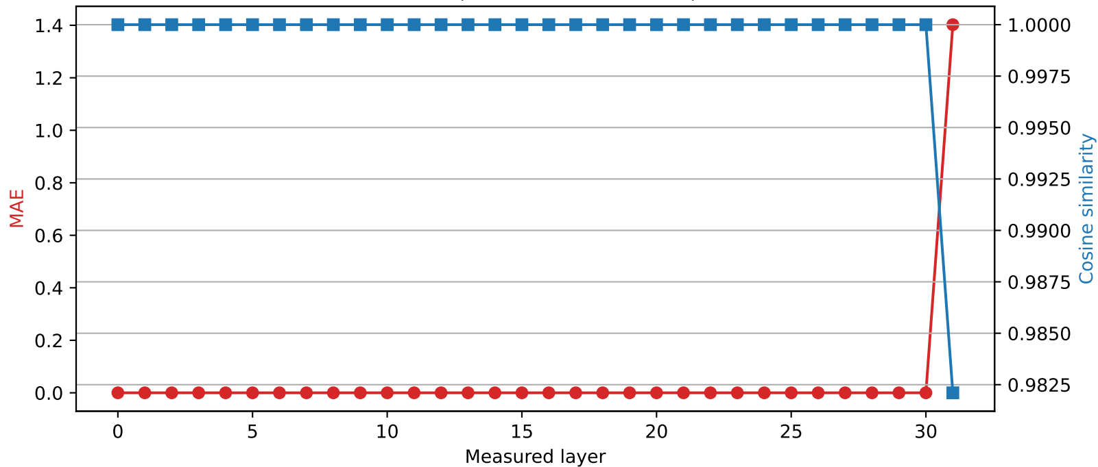
Phi-3-mini-4k-instruct | Quantized layer 30 | float32 \rightarrow int2
