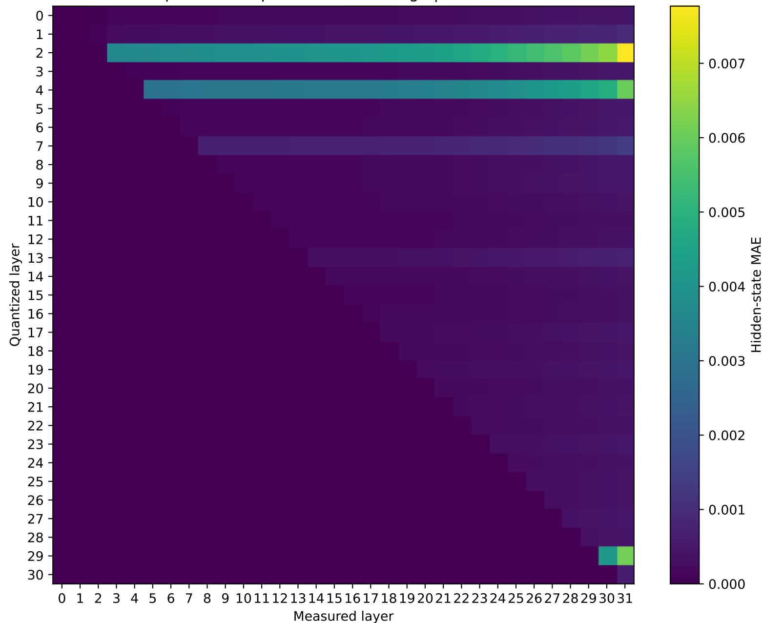
Phi-3-mini-4k-instruct Prompt 0: MAE representation damage | float64 → int16
