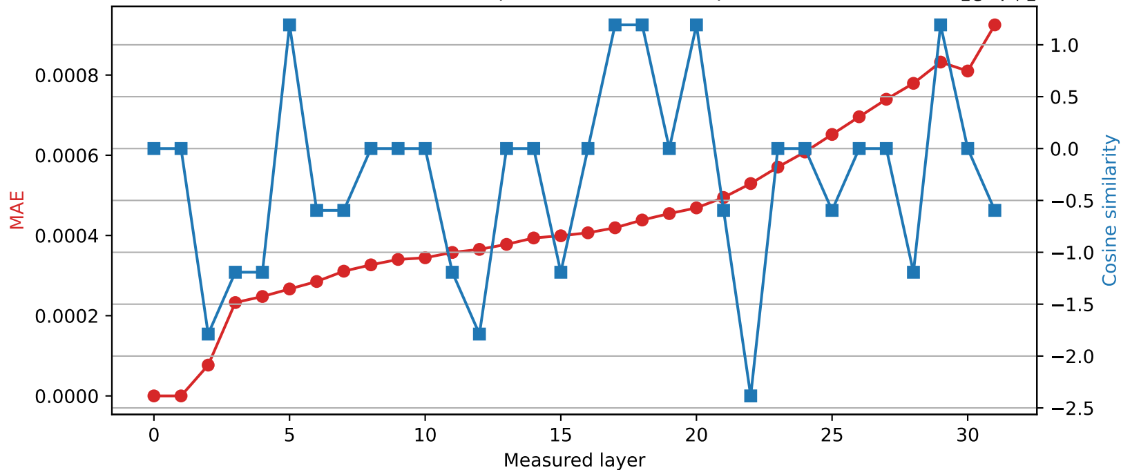
Phi-3-mini-4k-instruct | Quantized layer 1 | float64 → int16
