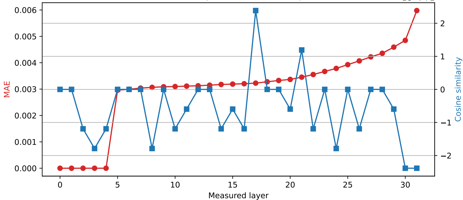
Phi-3-mini-4k-instruct | Quantized layer 4 | float64 → int16
