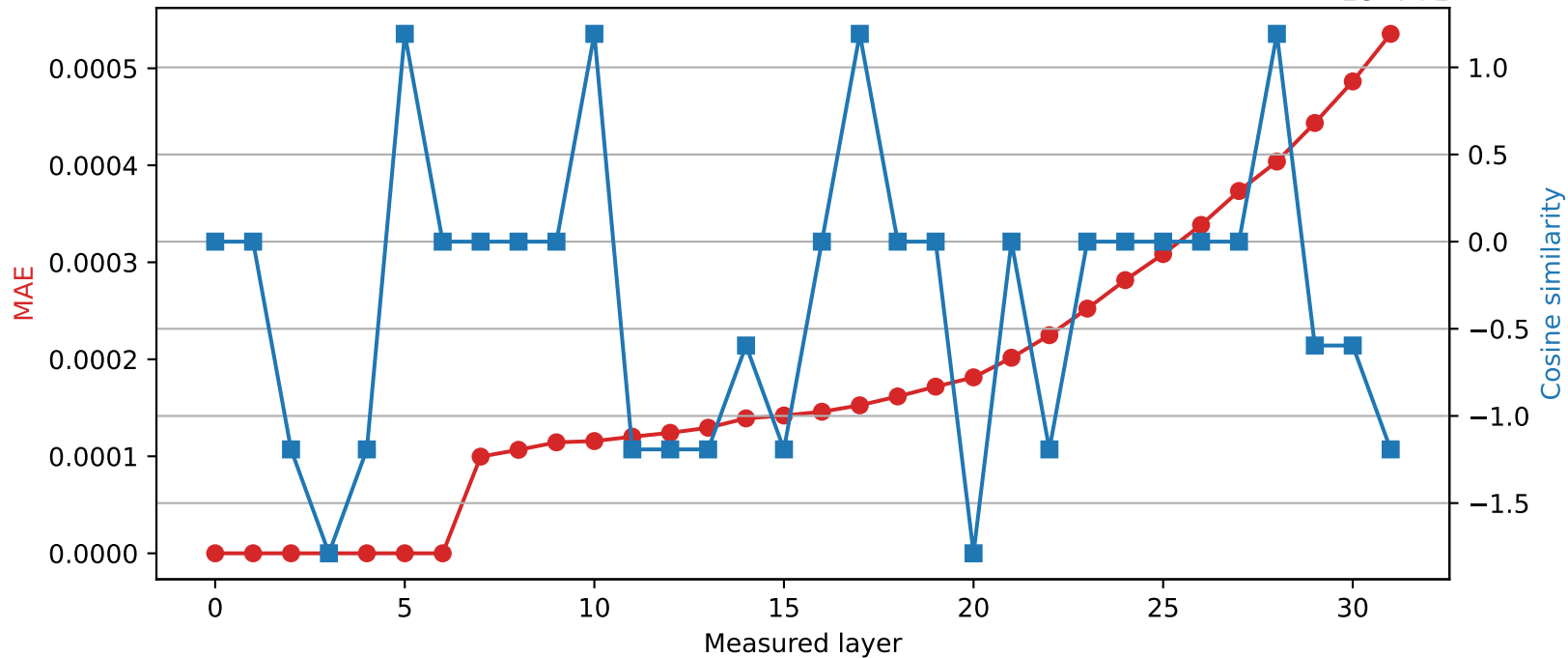
Phi-3-mini-4k-instruct | Quantized layer 6 | float64 → int16
