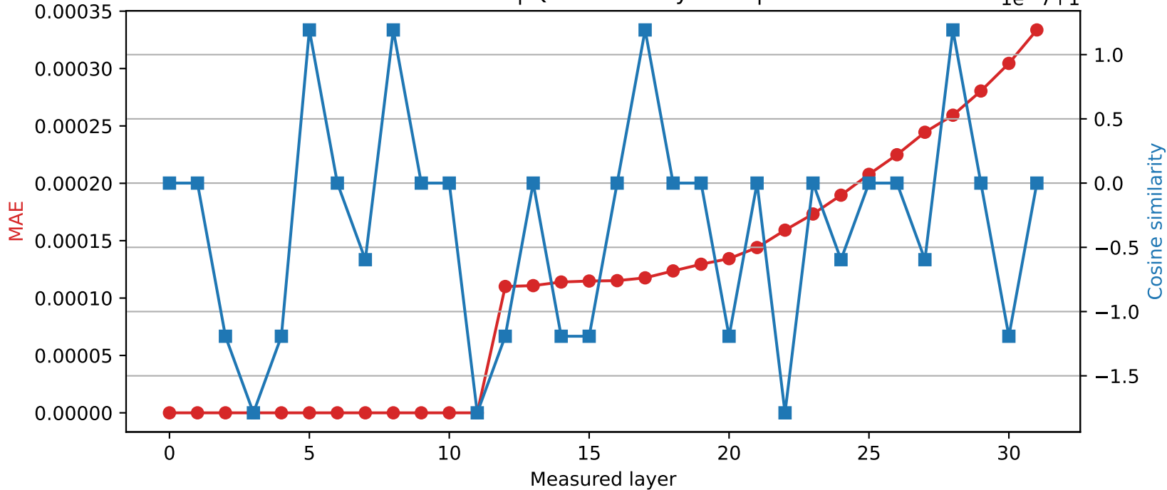
Phi-3-mini-4k-instruct | Quantized layer 11 | float64 \rightarrow int16
