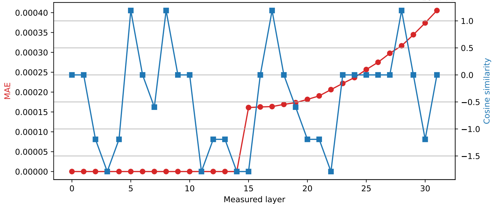
Phi-3-mini-4k-instruct | Quantized layer 14 | float64 \rightarrow int16
