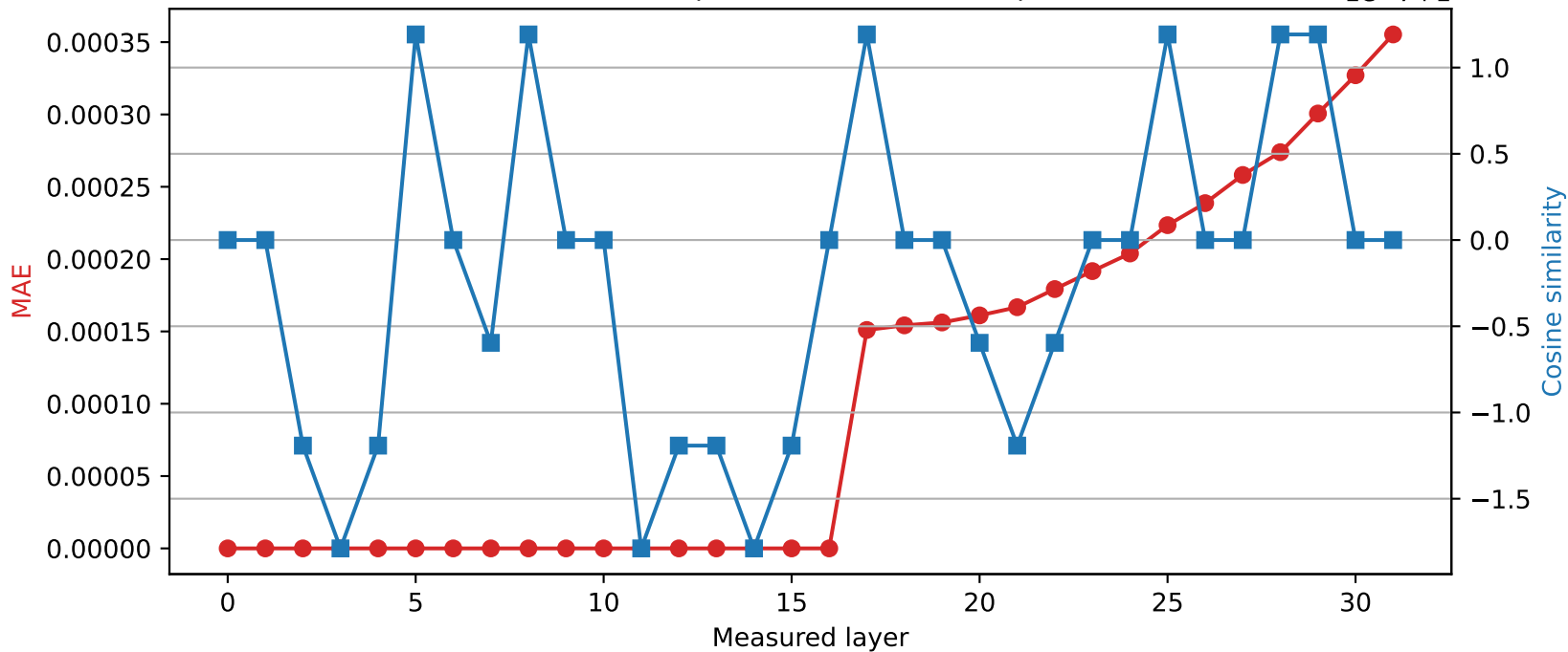
Phi-3-mini-4k-instruct | Quantized layer 16 | float64 \rightarrow int16
