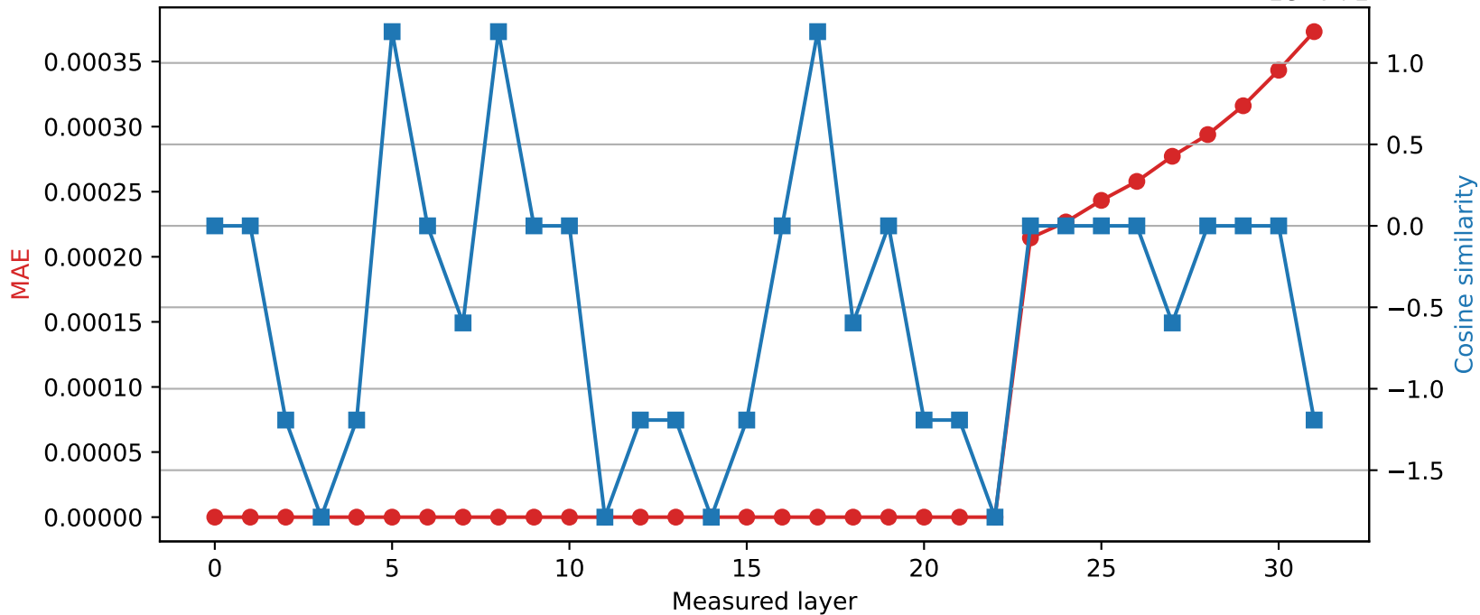
Phi-3-mini-4k-instruct | Quantized layer 22 | float64 \rightarrow int16
