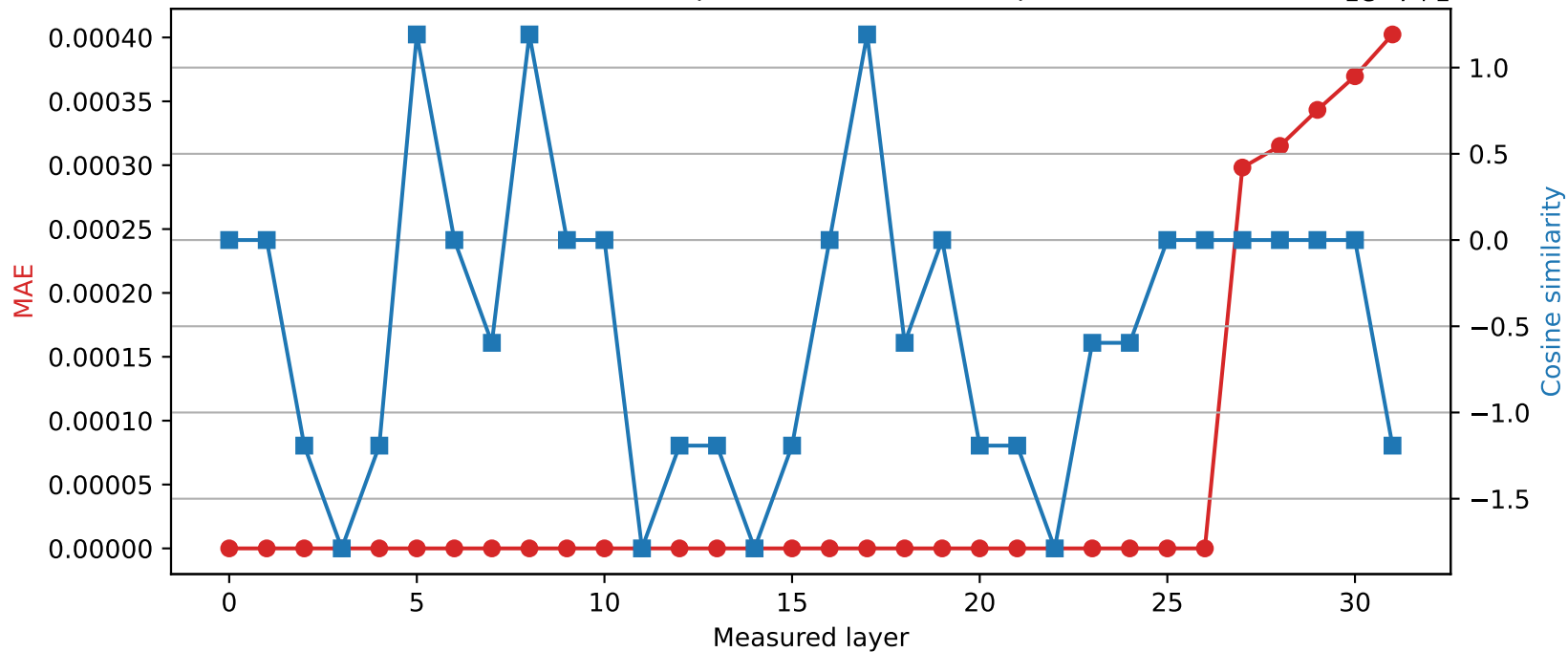
Phi-3-mini-4k-instruct | Quantized layer 26 | float64 \rightarrow int16
