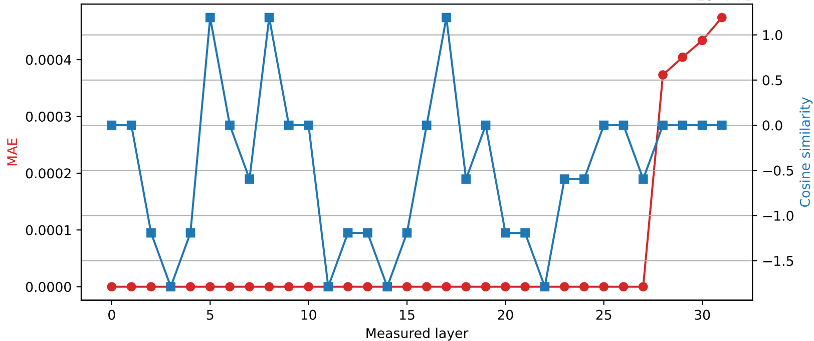
Phi-3-mini-4k-instruct | Quantized layer 27 | float64 \rightarrow int16
