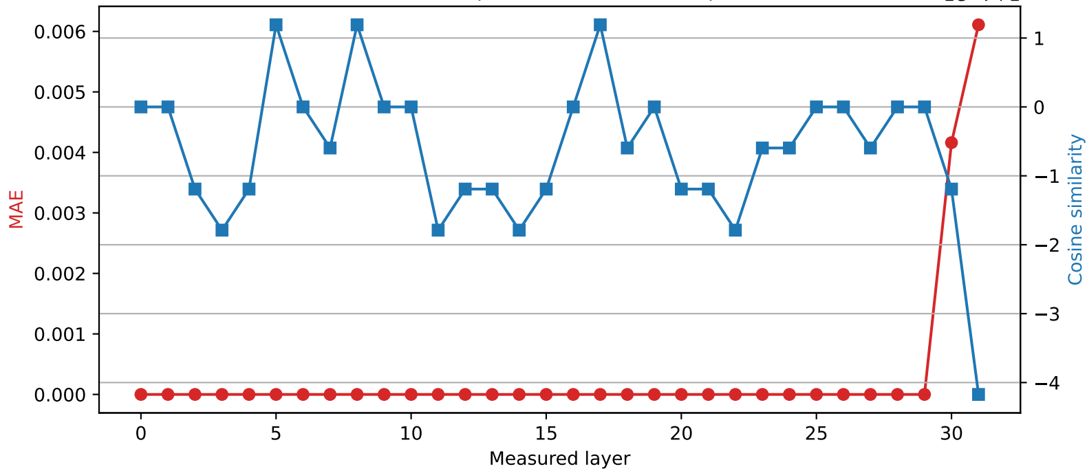
Phi-3-mini-4k-instruct | Quantized layer 29 | float64 \rightarrow int16
