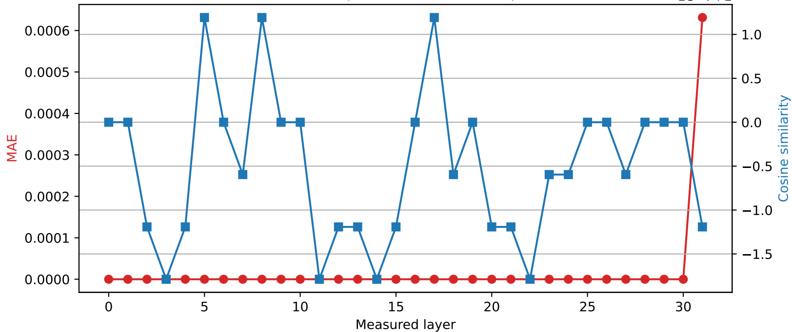
Phi-3-mini-4k-instruct | Quantized layer 30 | float64 \rightarrow int16
