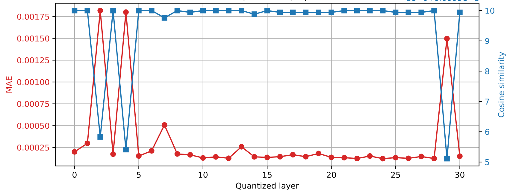
Phi-3-mini-4k-instruct | Prompt 1 Final RMSNorm output damage | float64 → int16
