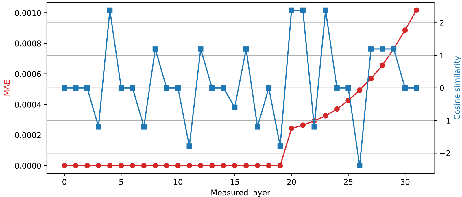
Phi-3-mini-4k-instruct | Quantized layer 19 | float64 \rightarrow int16
