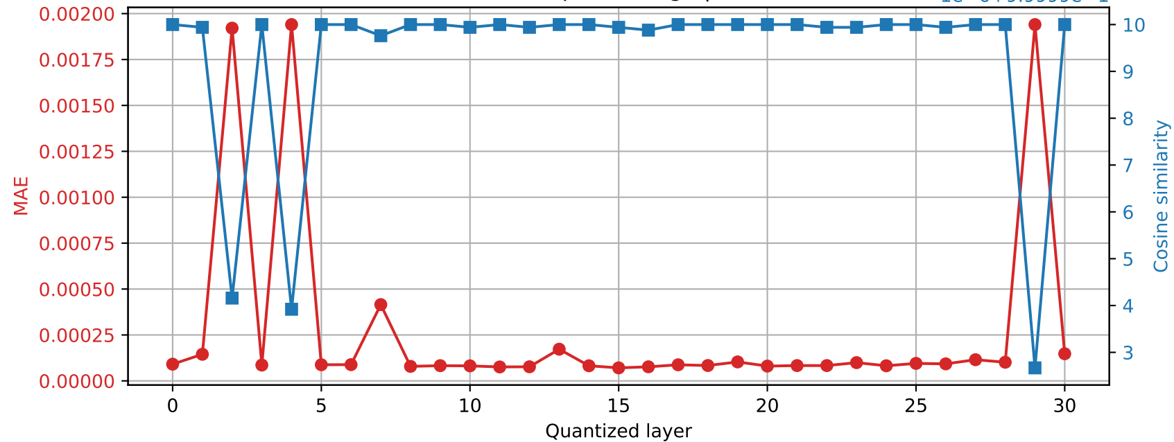
Phi-3-mini-4k-instruct | Prompt 2 Final RMSNorm output damage | float64 \rightarrow int16
