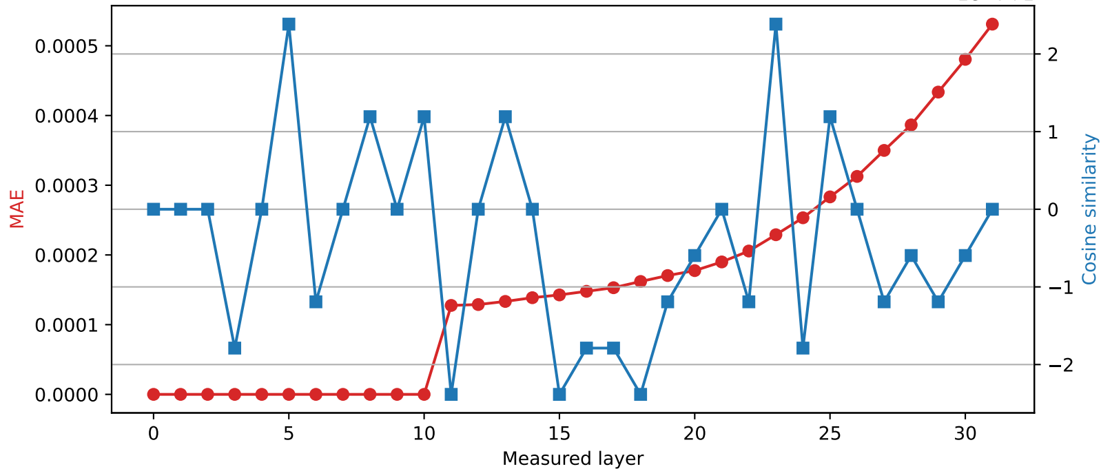
Phi-3-mini-4k-instruct | Quantized layer 10 | float64 \rightarrow int16
