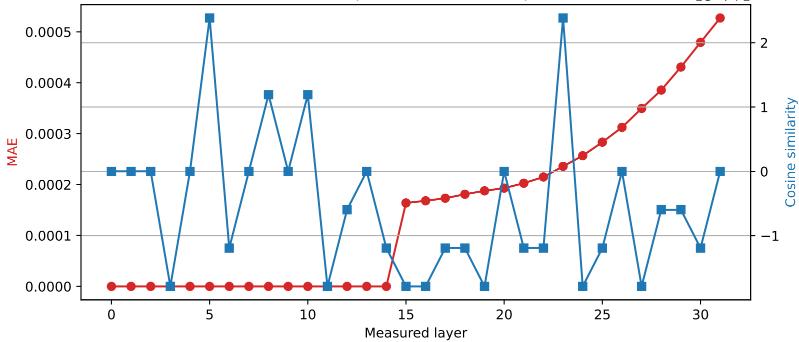
Phi-3-mini-4k-instruct | Quantized layer 14 | float64 \rightarrow int16
