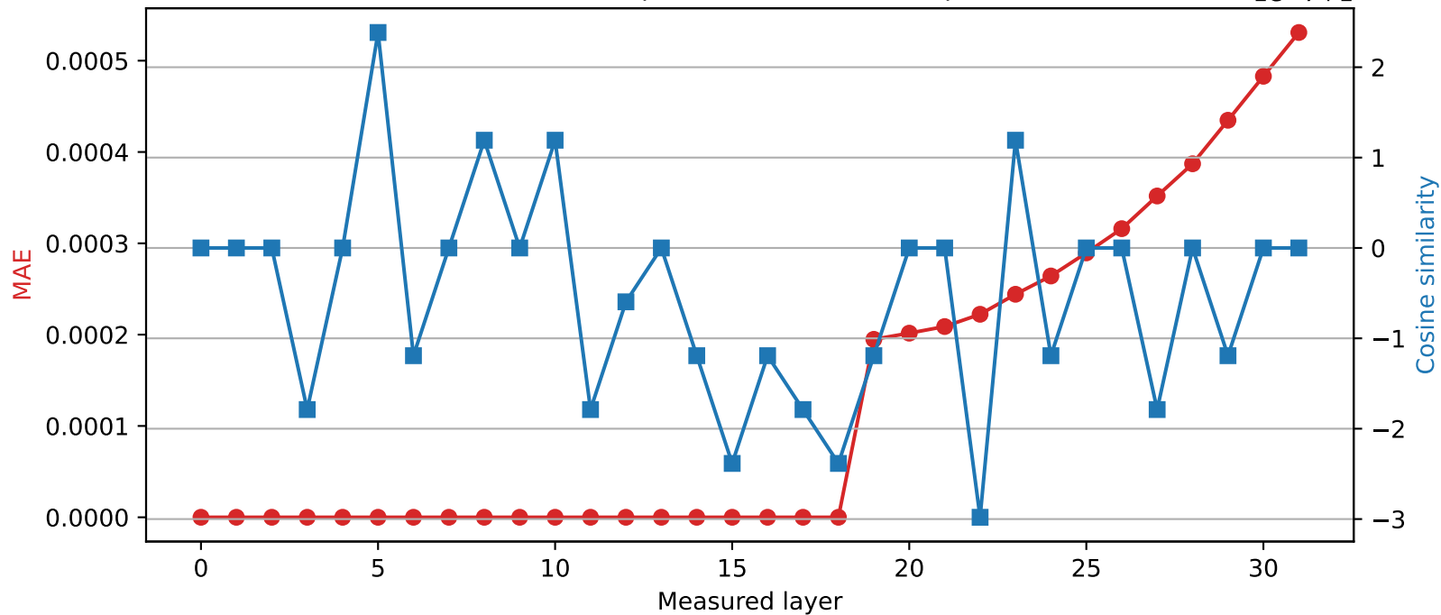
Phi-3-mini-4k-instruct | Quantized layer 18 | float64 → int16
