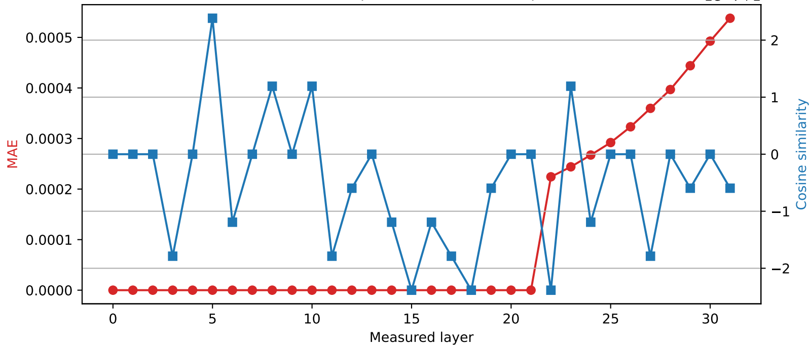
Phi-3-mini-4k-instruct | Quantized layer 21 | float64 \rightarrow int16
