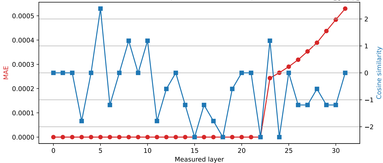
Phi-3-mini-4k-instruct | Quantized layer 22 | float64 \rightarrow int16
