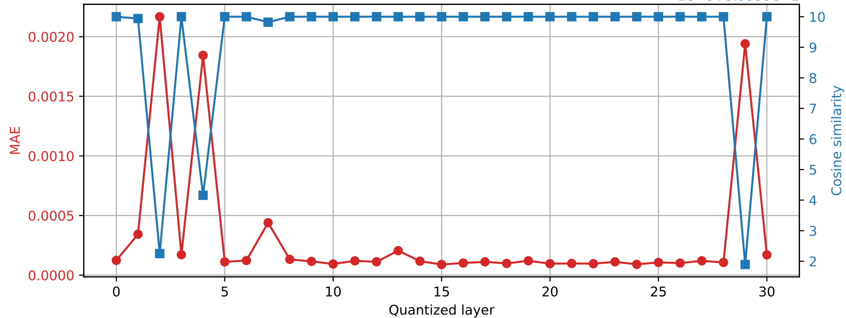
Phi-3-mini-4k-instruct | Prompt 3 Final RMSNorm output damage | float64 → int16
