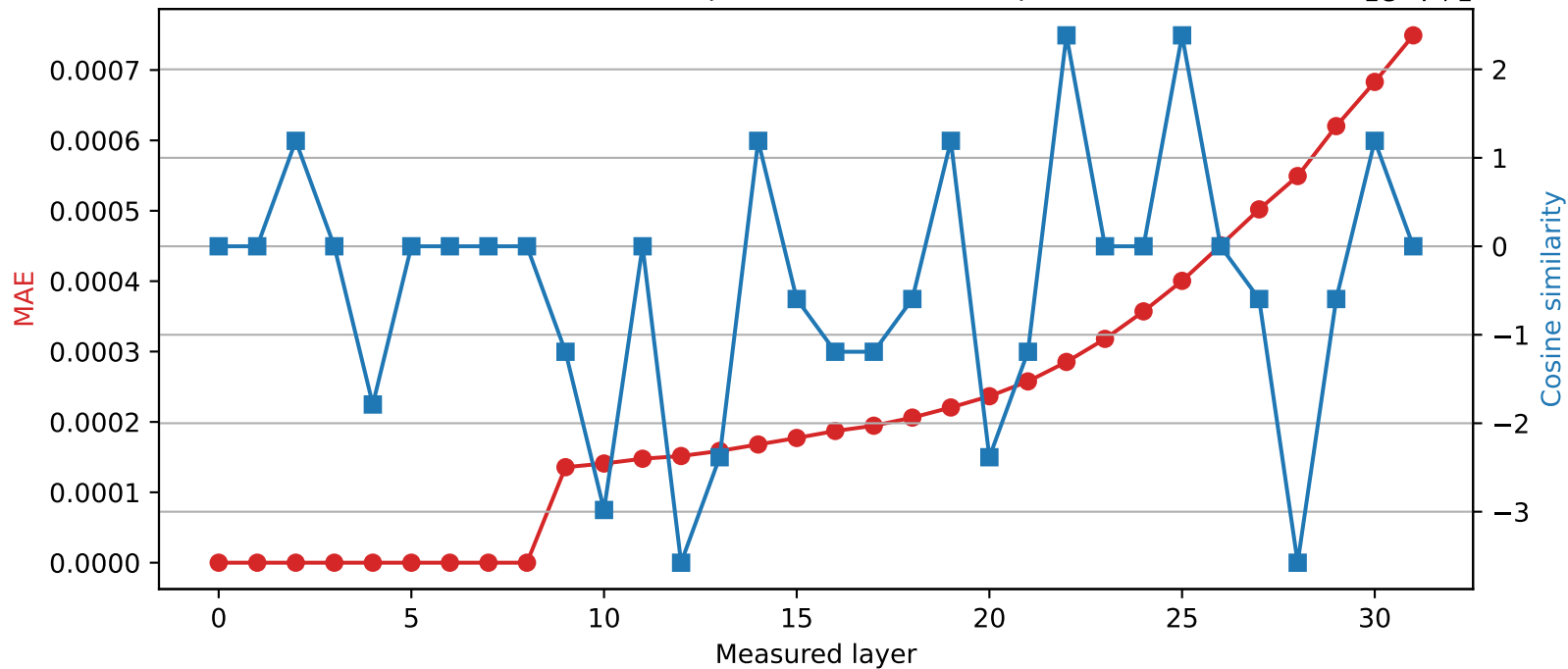
Phi-3-mini-4k-instruct | Quantized layer 8 | float64 → int16
