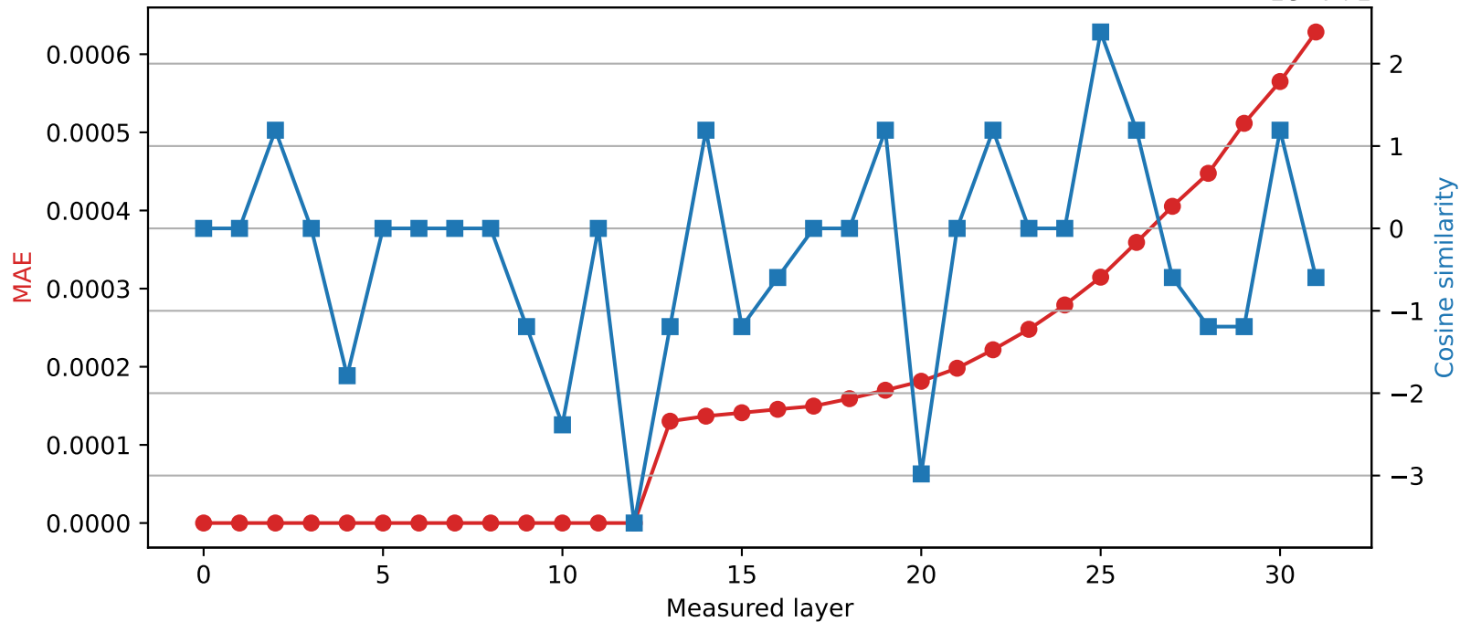
Phi-3-mini-4k-instruct | Quantized layer 12 | float64 \rightarrow int16
