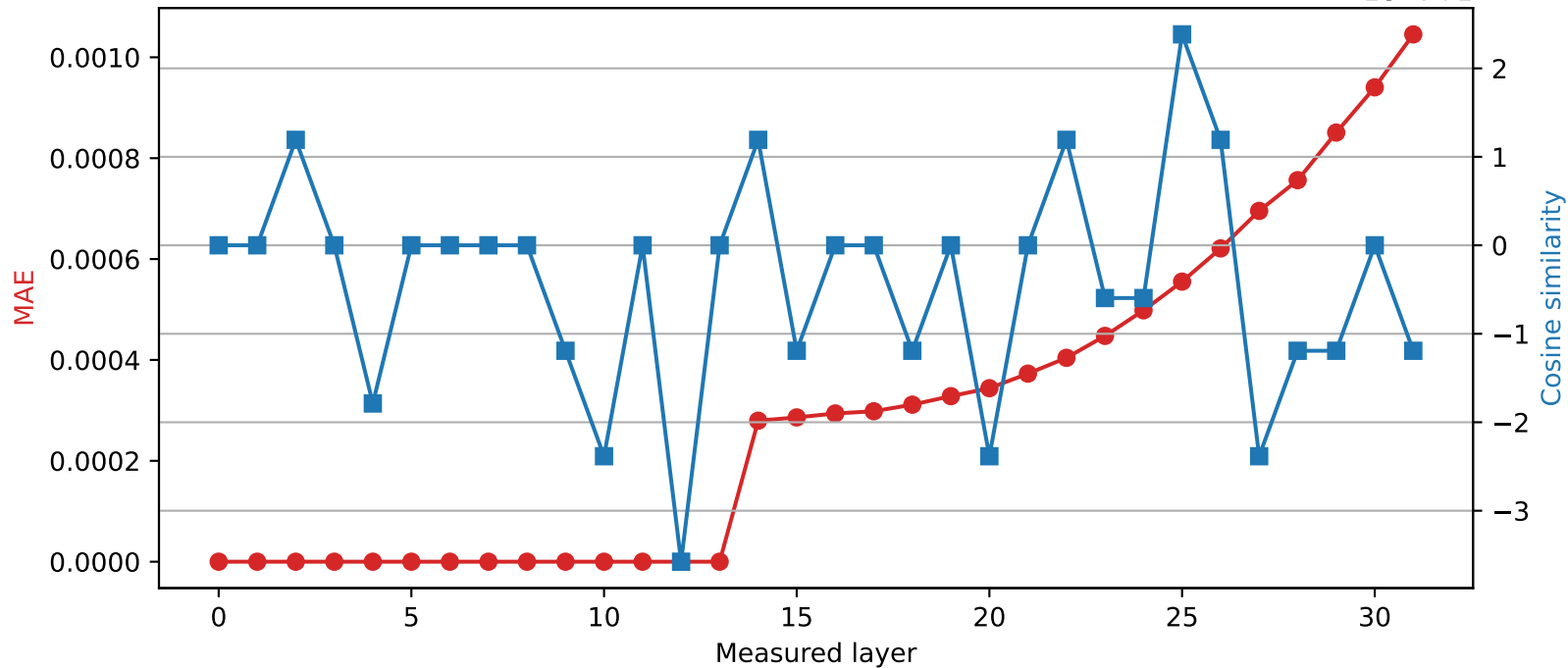
Phi-3-mini-4k-instruct | Quantized layer 13 | float64 → int16
