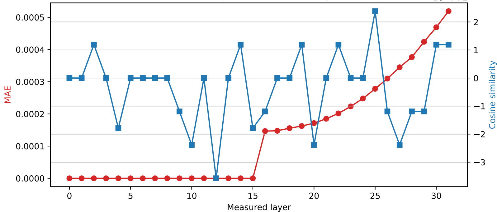
Phi-3-mini-4k-instruct | Quantized layer 15 | float64 \rightarrow int16
