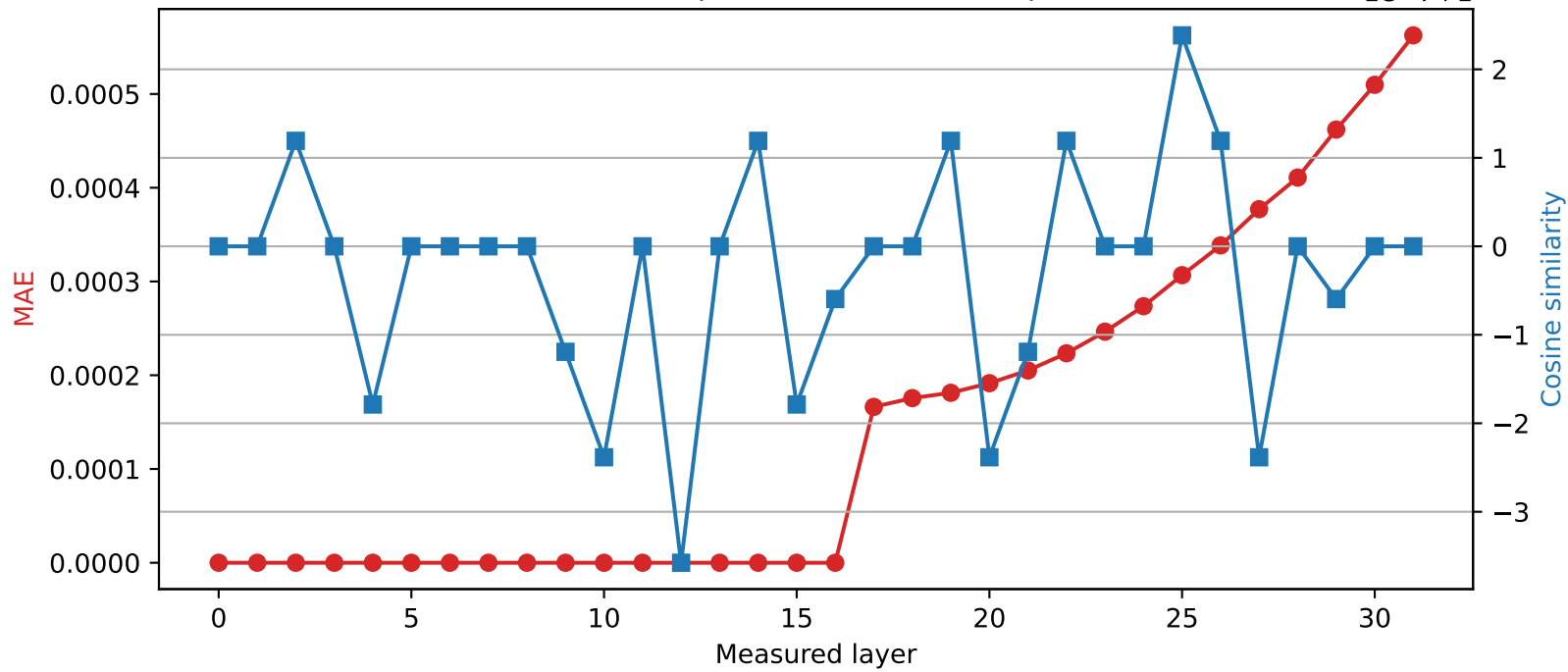
Phi-3-mini-4k-instruct | Quantized layer 16 | float64 \rightarrow int16
