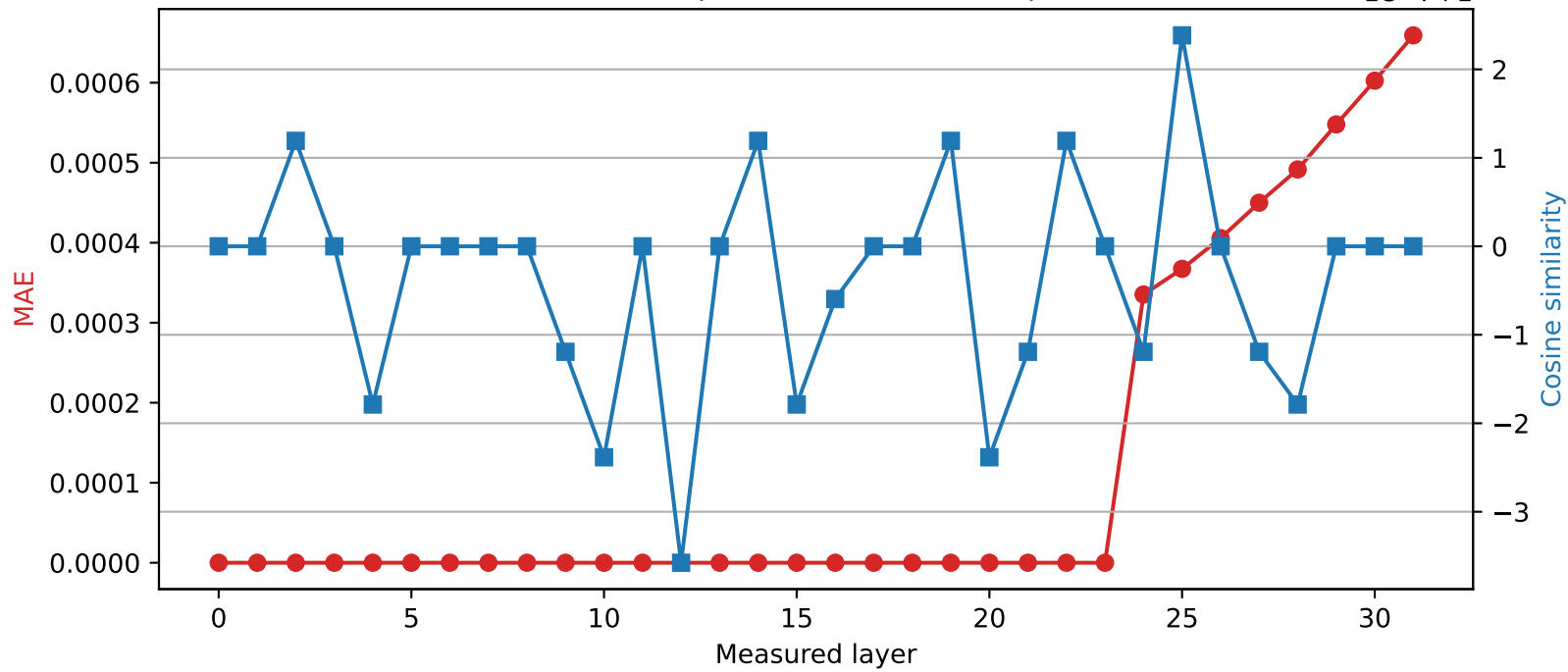
Phi-3-mini-4k-instruct | Quantized layer 23 | float64 \rightarrow int16
