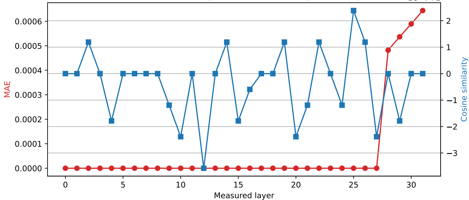
Phi-3-mini-4k-instruct | Quantized layer 27 | float64 \rightarrow int16
