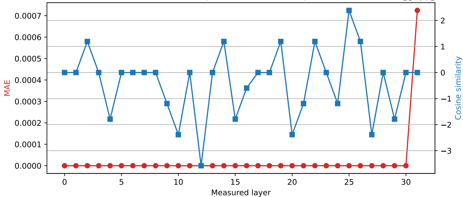
Phi-3-mini-4k-instruct | Quantized layer 30 | float64 \rightarrow int16
