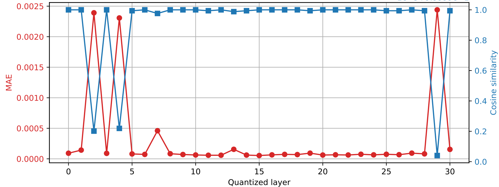
Phi-3-mini-4k-instruct | Prompt 4 Final RMSNorm output damage | float64 → int16
