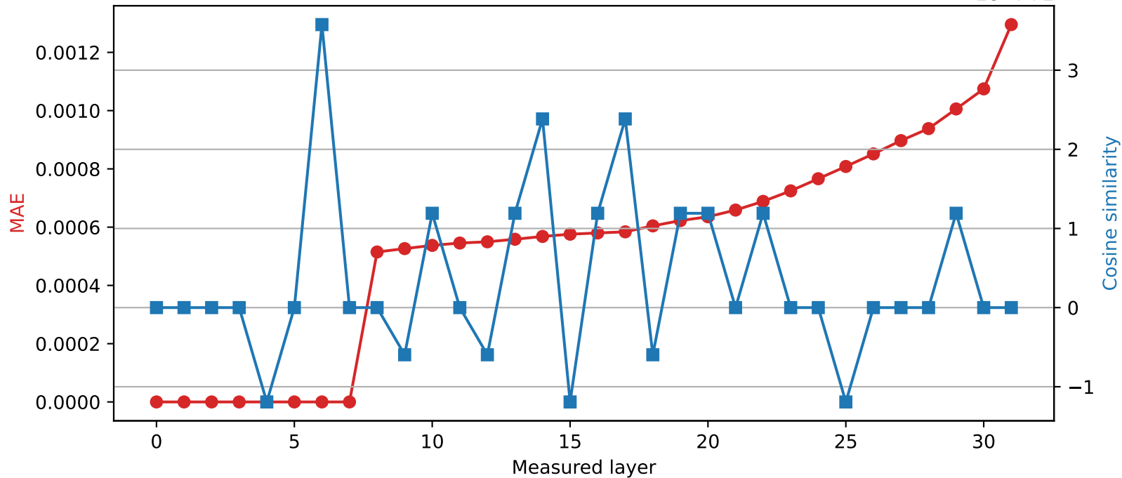
Phi-3-mini-4k-instruct | Quantized layer 7 | float64 → int16
