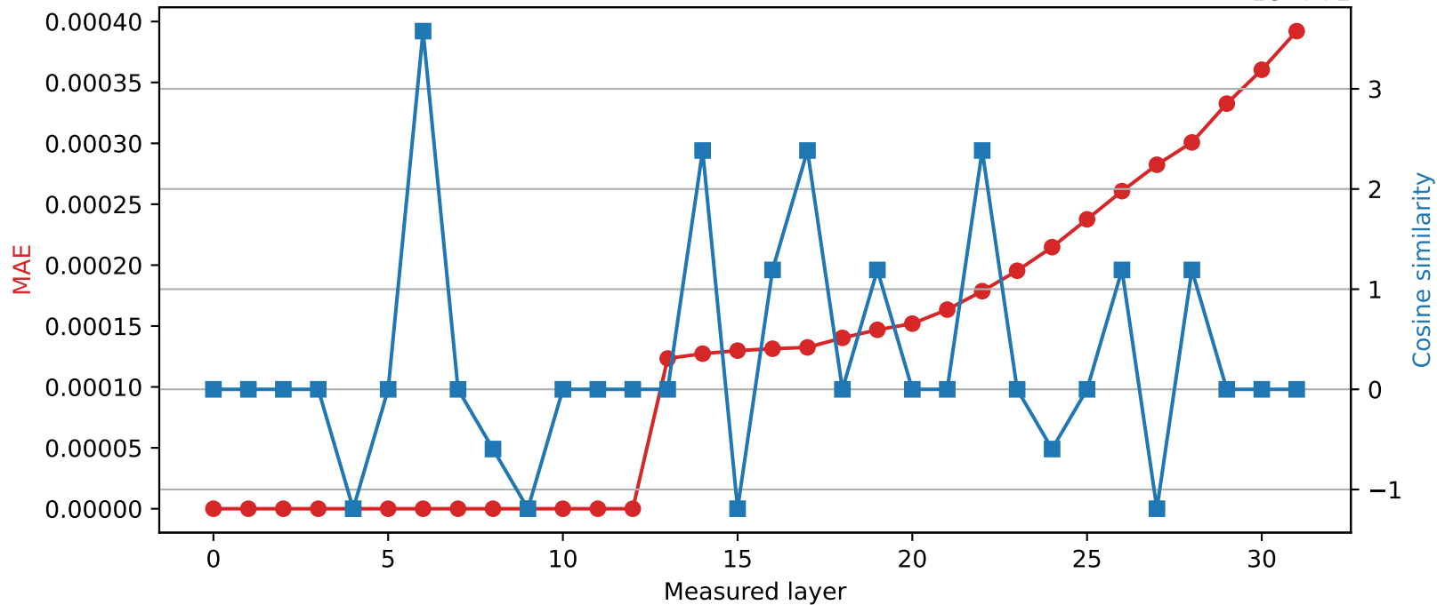
Phi-3-mini-4k-instruct | Quantized layer 12 | float64 → int16
