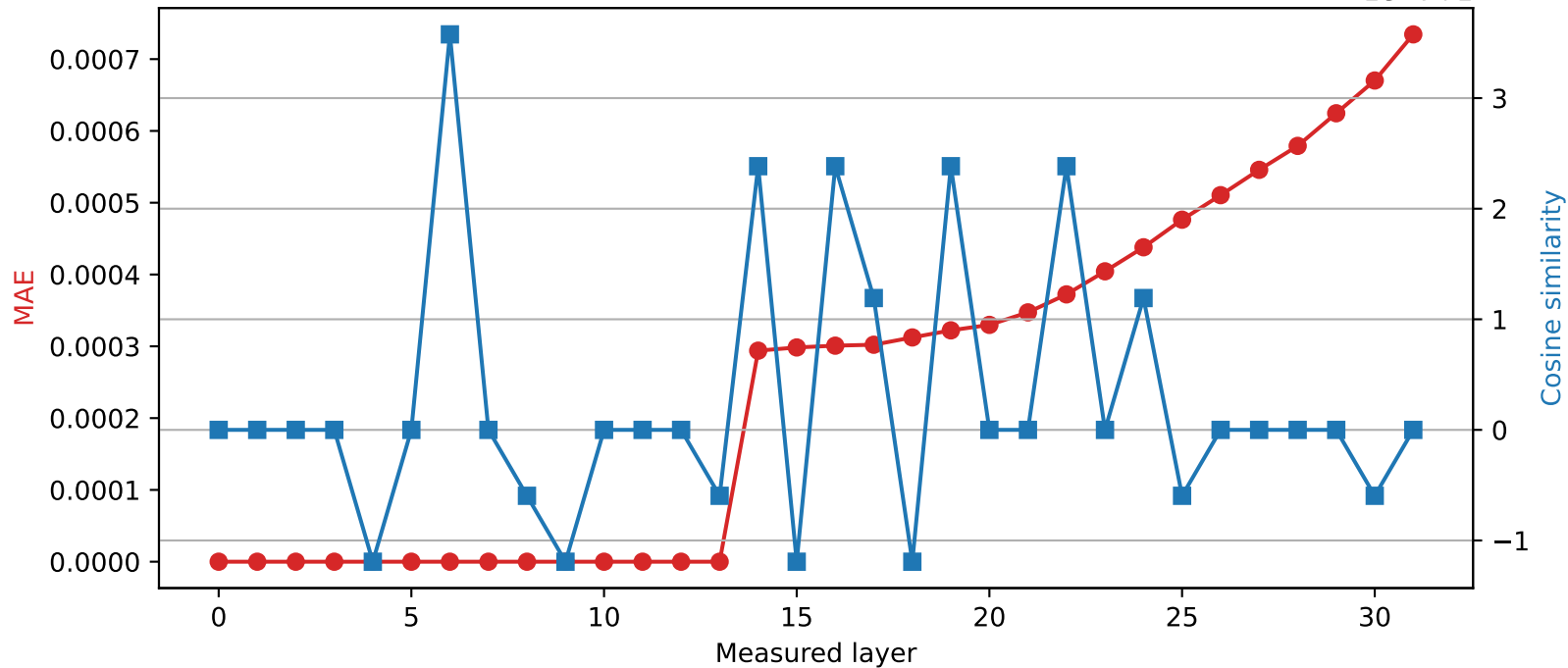
Phi-3-mini-4k-instruct | Quantized layer 13 | float64 \rightarrow int16
